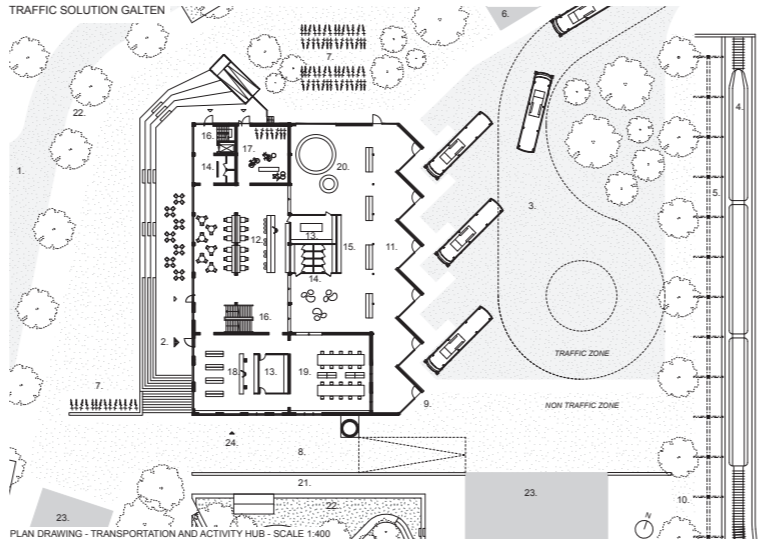
PLAN DRAWING - TRANSPORTATION AND ACTIVITY HUB - SCALE 1:400
