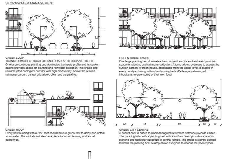
PLAN DRAWING - SQUARE AND GARDEN BLOCK - SCALE 1:400
