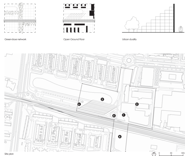
Site plan
