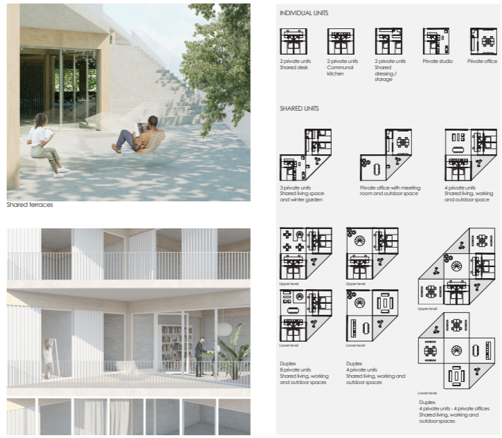
Shared terraces
